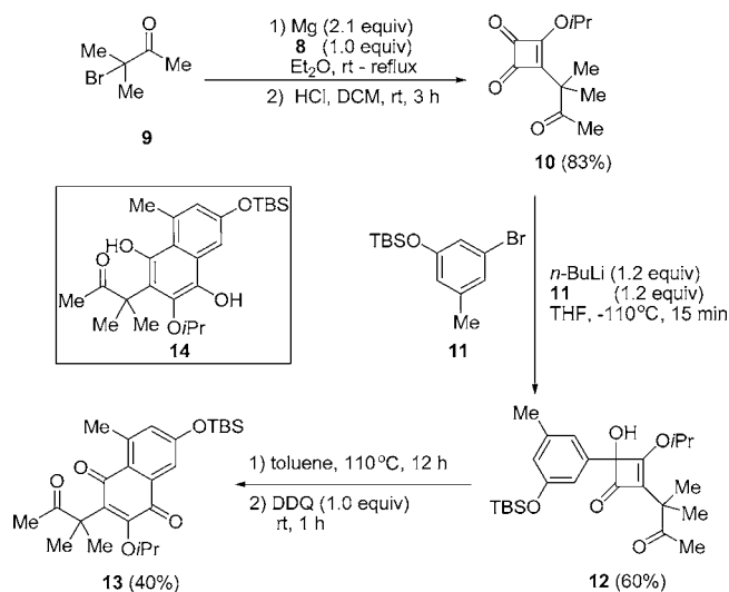
Scheme 2. Synthesis and Ring Expansion of 12
