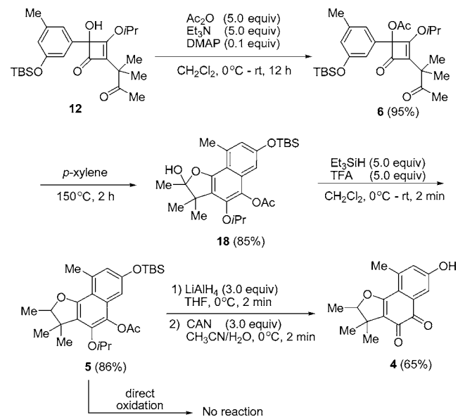
Scheme 4. Synthesis of 4
