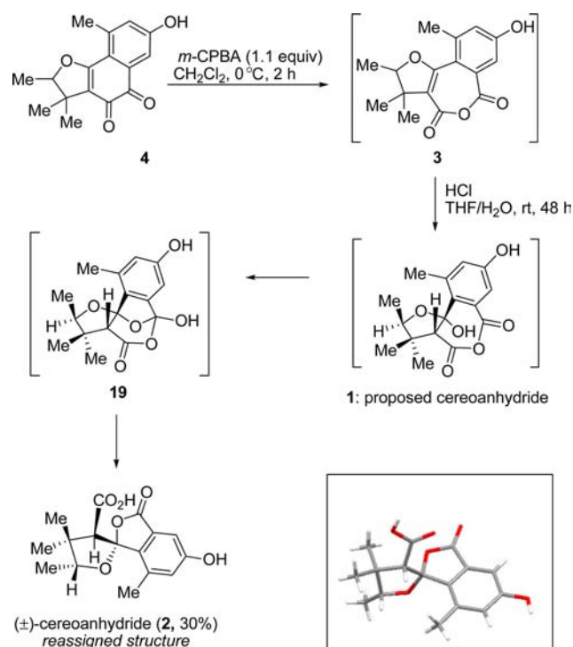
Scheme 5. Synthesis and Structural Reassignment of Cereoanhydride
