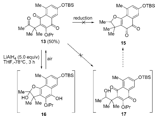
Scheme 3. Reduction of 13
