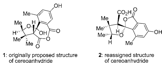
Figure 1. Structures of originally proposed and reassigned cereoanhydride.
